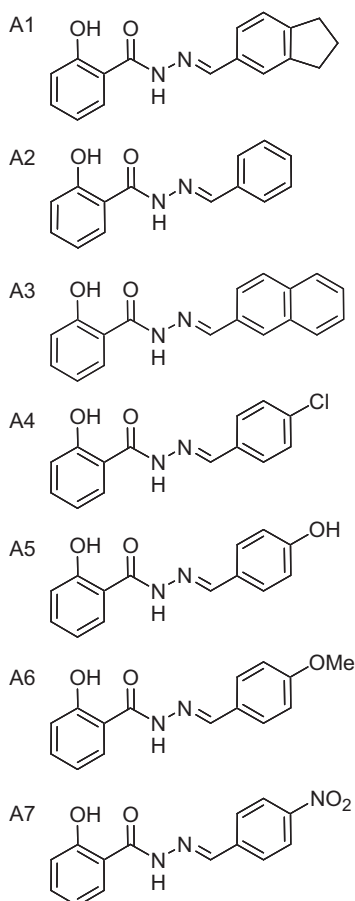
Figure 2. Hydrazide analogs.
