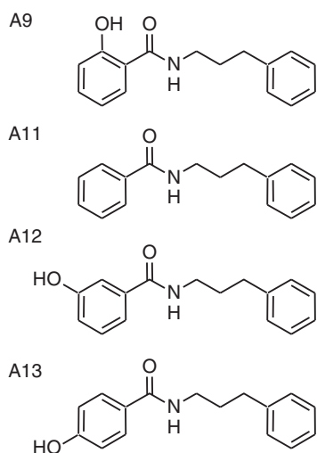
Figure 4. Benzamide analogs.
