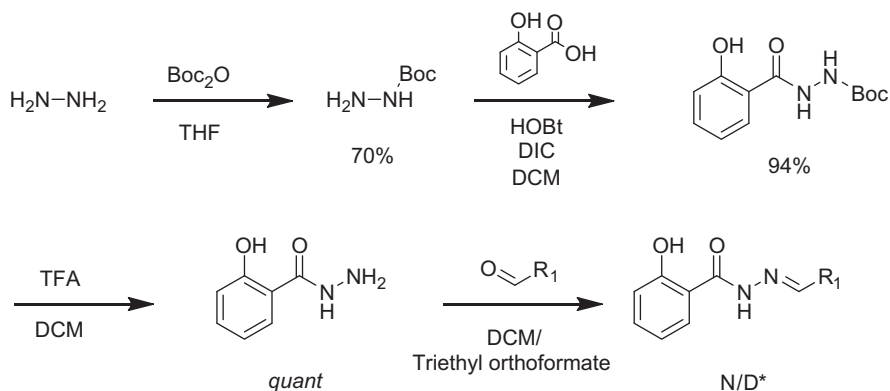
Figure 2. Hydrazide analogs.
