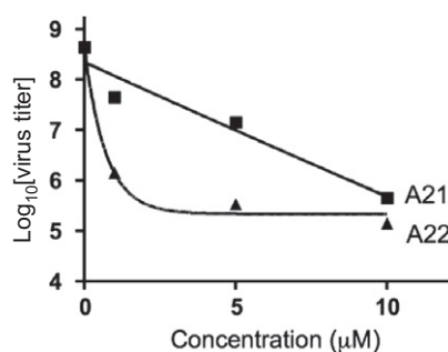
Figure 5. Phenylpropylamide analogs.
